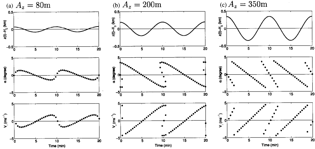
Fig. 6. Simulation results of the reflecting point and radial velocity when a partial reflecting layer is modulated by a deep sinusoidal wave, whose horizontal wavelength is 20 km, advected through a vertically pointing radar beam. The mean altitude of the displacement of the distorted layer is at 88 km with a radar beamwidth of 7.8^\circ corresponding to a horizontal coverage of approximately 12 km. The period of the wave is 10 min and the amplitude of the wave is (a) 80 m, (b) 200 m, and (c) 350 m. When the vertical displacement of modulated layer becomes larger as shown in (b) and (c), multiple reflecting points and spectral features can be observed when the crest of the wave is at zenith. In (c), the diagonal hatching and overlapping structures of \alpha and V_r are exhibited when the wave is significantly steepened.
