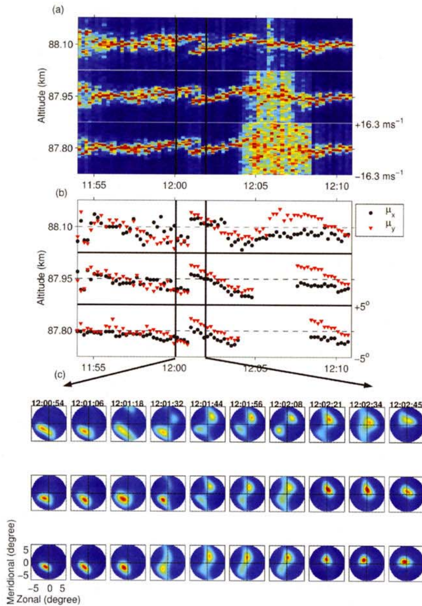
Fig. 4. Composite plot of results from Case I of frequency jumps/overlapping. The spectrograms are shown in (a) for three adjacent heights (87.8, 87.95, and 88.1 km). The angular location of the peak of individual brightness estimates in the zonal and meridional directions are denoted by \mu_x and \mu_y , respectively, and are shown in (b). Individual values of \mu_x and \mu_y are denoted by black circles and red triangles, respectively. The missing \mu_x and \mu_y are those data whose SNR are less than -5 dB. The brightness estimates shown in (c) are for the marked region where the frequency jumps are present. Each brightness estimate ( 64 \times 64 pixels) is made from -7^\circ to 7^\circ in both zonal and meridional directions every 12 s at each gate using Capon CRI. The results of CRI show that a double-peak structure exists during the frequency jump/overlapping period with single-peak, opposing structures appearing before and after the jumps.
