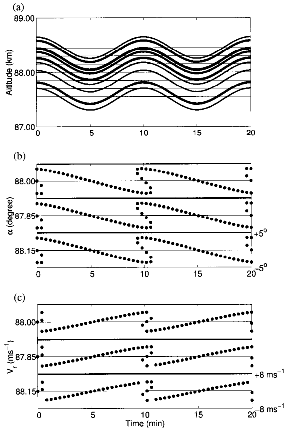
Fig. 7. Simulation of multiple layers which are synchronously modulated by a deep sinusoidal wave. As a result, multiple reflecting points and overlapping features in radial velocity occur at several gates. The 15 layers are randomly distributed over approximately 1 km (87.5–88.5 km). The modulating wave has a horizontal wavelength and vertical amplitude of 20 km and 200 m, respectively. Seven range gates with 150 m resolution (thin solid lines) are used to determine in which gate the glint angles exist. The middle and bottom plots are the average glint angle and radial velocity observed in the middle three gates.
