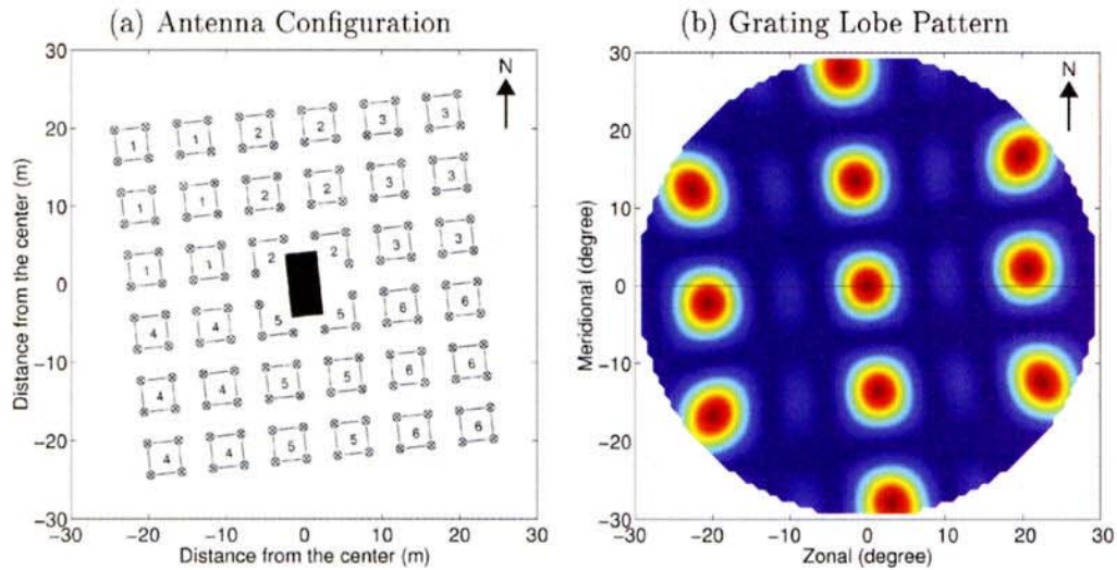
Fig. 1. (a) Antenna configuration of the ESRAD system. The number in each group of four Yagi antennas denotes the receiver to which they are connected. (b) The grating lobe pattern, which is derived based on (a), is plotted from -30^\circ to 30^\circ in both the zonal and meridional directions. All grating lobes are at least 15^\circ away from the origin.
