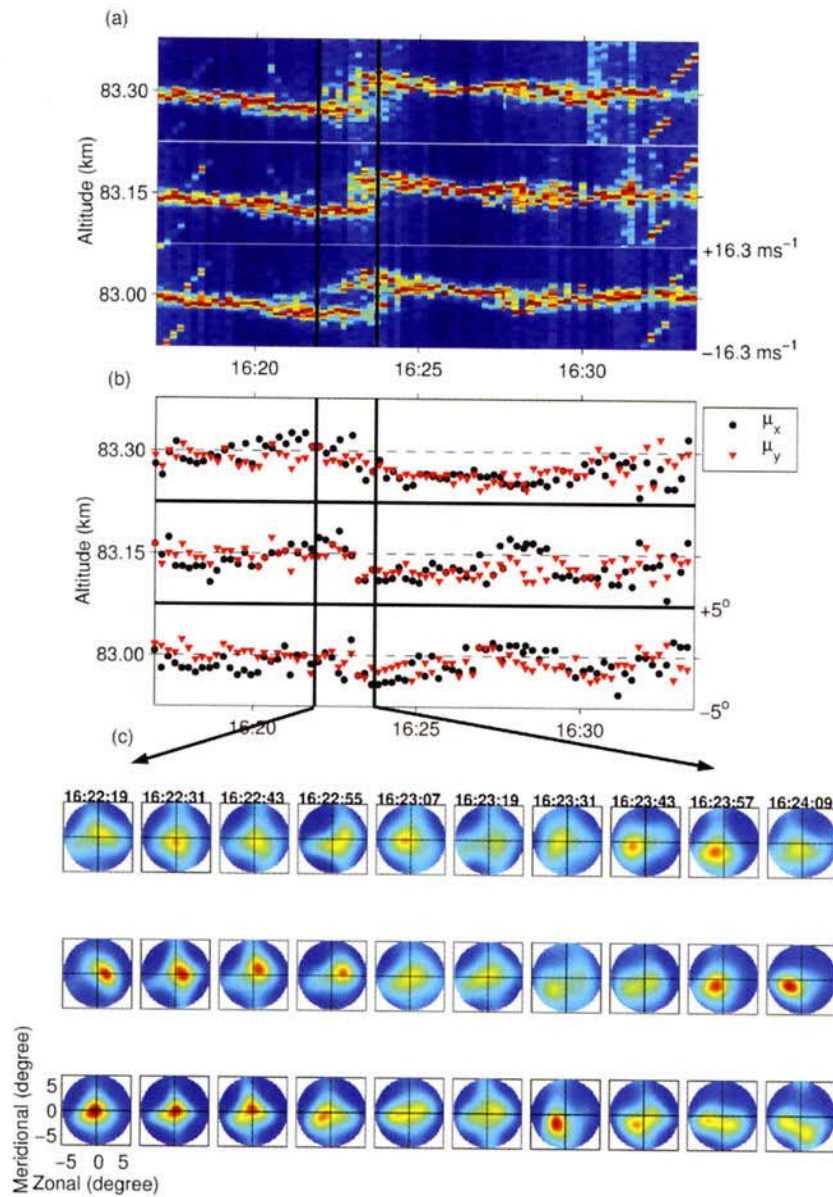
Fig. 5. Composite plot of results from Case II of frequency jumps/overlapping. Same as previous figure except for the time from 1615 to 1635 UT and altitudes of 83.0, 83.15, and 83.3 km. In this case, Capon CRI does not seem to have enough resolution to resolve the double-peak structure during the frequency jumps/overlapping. Nevertheless, the locations of the single-peak structures still do jump to the opposite side at the time of the frequency jumps.
