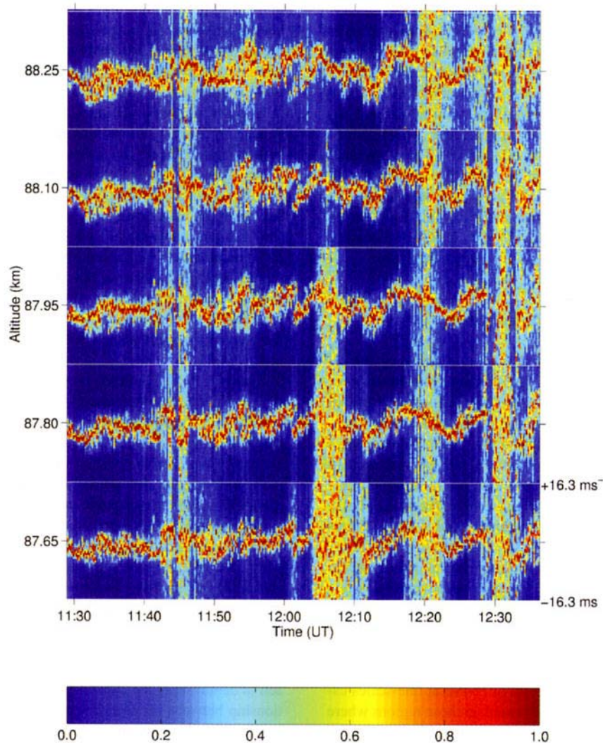
Fig. 3. An example of spectrograms from five range gates and approximately 1 h of elapsed time. Individual spectra are self-normalized at each height and have an aliasing velocity of 16.34 \text{ m s}^{-1} . Diagonal hatching and overlapping structures can be observed in the middle three gates at approximately 1200 UT followed by a disappearance of the signals for a 3-min period. Subsequently, cusp features can be seen at 1215 and 1225 UT.
