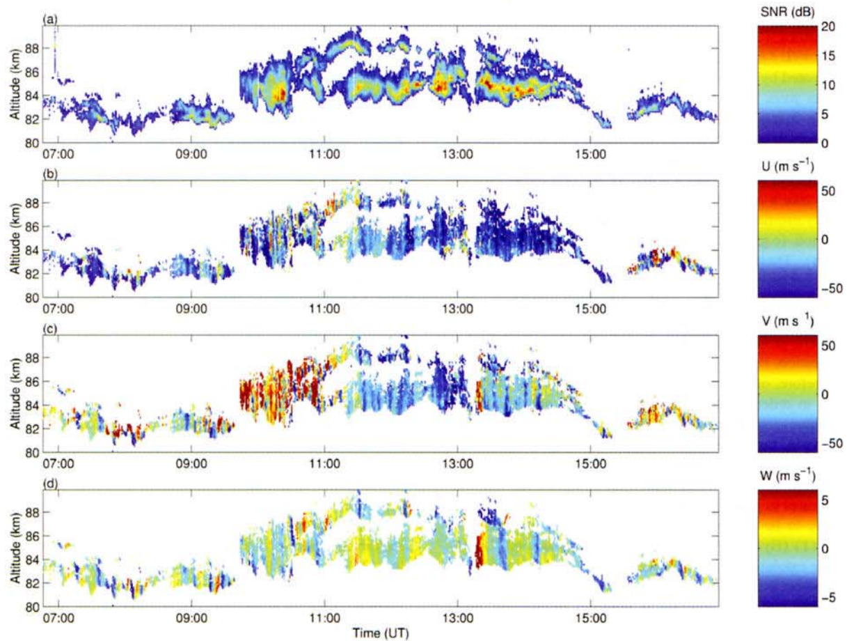
Fig. 2. Range-time intensity plots of (a) SNR, (b) zonal, (c) meridional, and (d) vertical velocity of a 10-h period on August 3, 1998.
