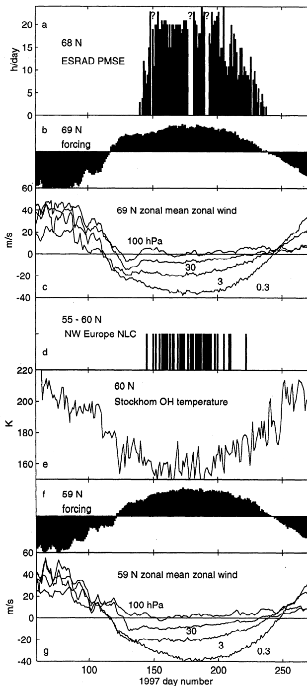
Figure 1. Seasonal variation during 1997 of: a: PMSE measured by ESRAD (? indicates data gap); b forcing in the mesosphere calculated from the stratospheric winds in c (see text for details); c - stratospheric zonal winds at 69°N for the 100, 30, 3 and 0.3 hPa pressure levels (approx. 16, 24, 40 and 60 km altitude) from the UKMO-UARS assimilation d - nights when noctilucent clouds were observed from Britain and northern Europe; e - OH temperatures at 86+4 km measured at Stockholm; f and g as panels b and c, but for 59°N.
