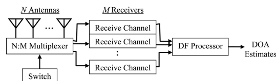
Fig. 1. Block diagram of switched-element DF system.
